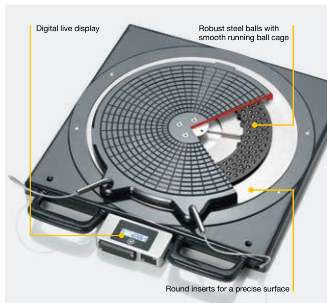
Digital corner weight scales: Turntables equipped with high-precision load cells enable weight distribution to be integrated directly into the wheel alignment.
